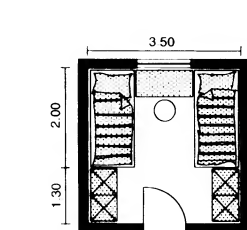
⑭ Two-bed room for children/guests
